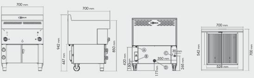
GHPI 7/700
