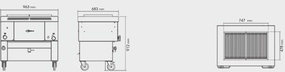
GHPI 2F/1000
