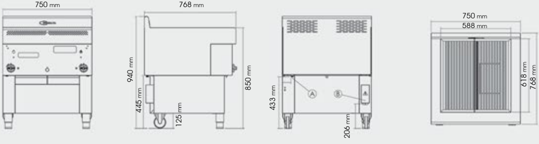
GHPI 2/600
