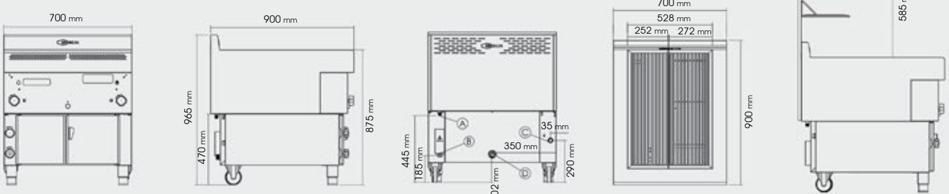
GHPI 2/750
