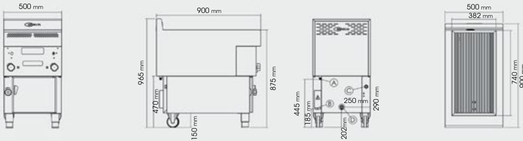
GHPI 2/700
