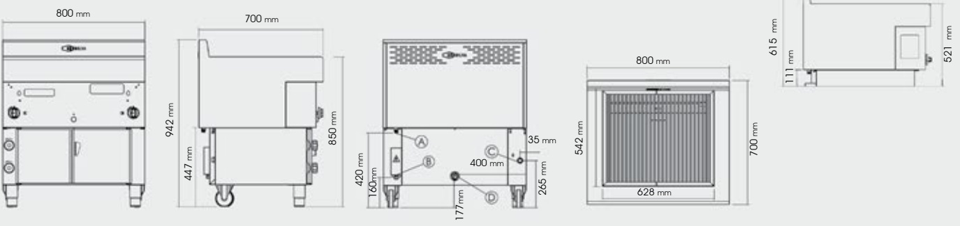
GHPI 7/800
