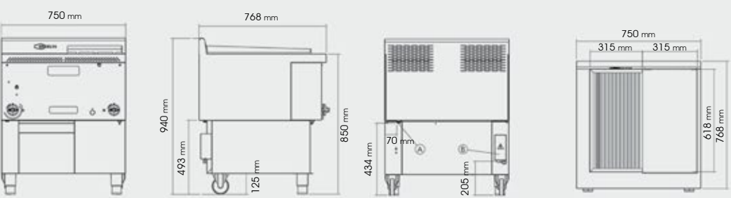
GHPI C2/6
