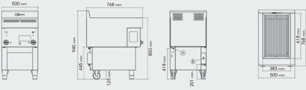
GHPI 2/500
